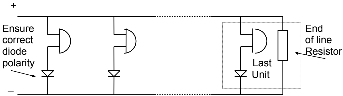
Fig. 1.1 Typical sounder circuit
