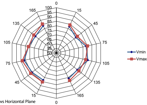
Tone 20 Angular Performance (dB(A) at 1m)
