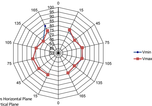
Voice Message 1 Angular Performance (dB(A) at 1m)
