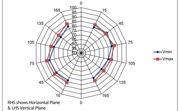
Tone 6 Angular Performance (dB(A) at 1m)
