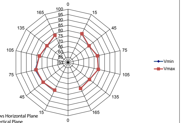
Voice Message 3 Angular Performance (dB(A) at 1m)
