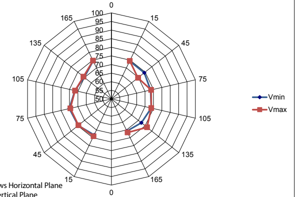
Voice Message 2 Angular Performance (dB(A) at 1m)
