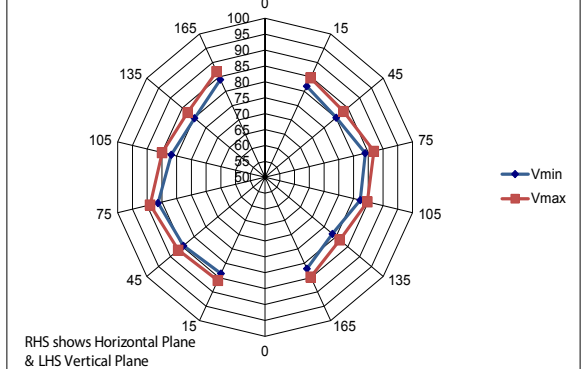
Tone 15 Angular Performance (dB(A) at 1m)
