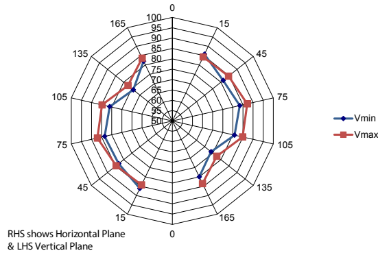
Tone 1 Angular Performance (dB(A) at 1m)
