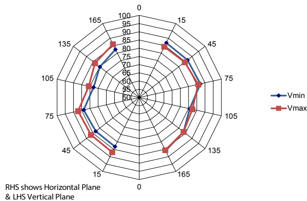
Tone 3 Angular Performance (dB(A) at 1m)
